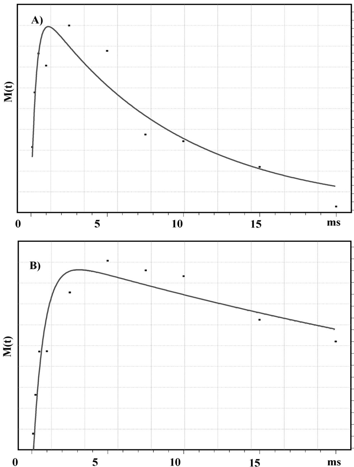
Figure 10: ^{13}\text{C} CP/MAS variable-contact data (magnetization plotted in arbitrary units) for carbon 2 (aromatic \text{NH}_2 -bearing carbon; see Fig. 1(B)) resonance in a sample containing ^{14}\text{N} at natural abundance (A) and of a sample highly enriched in ^{15}\text{N} (B). The smooth line in each is a fit to Mehring's variable-contact model. (See text).
