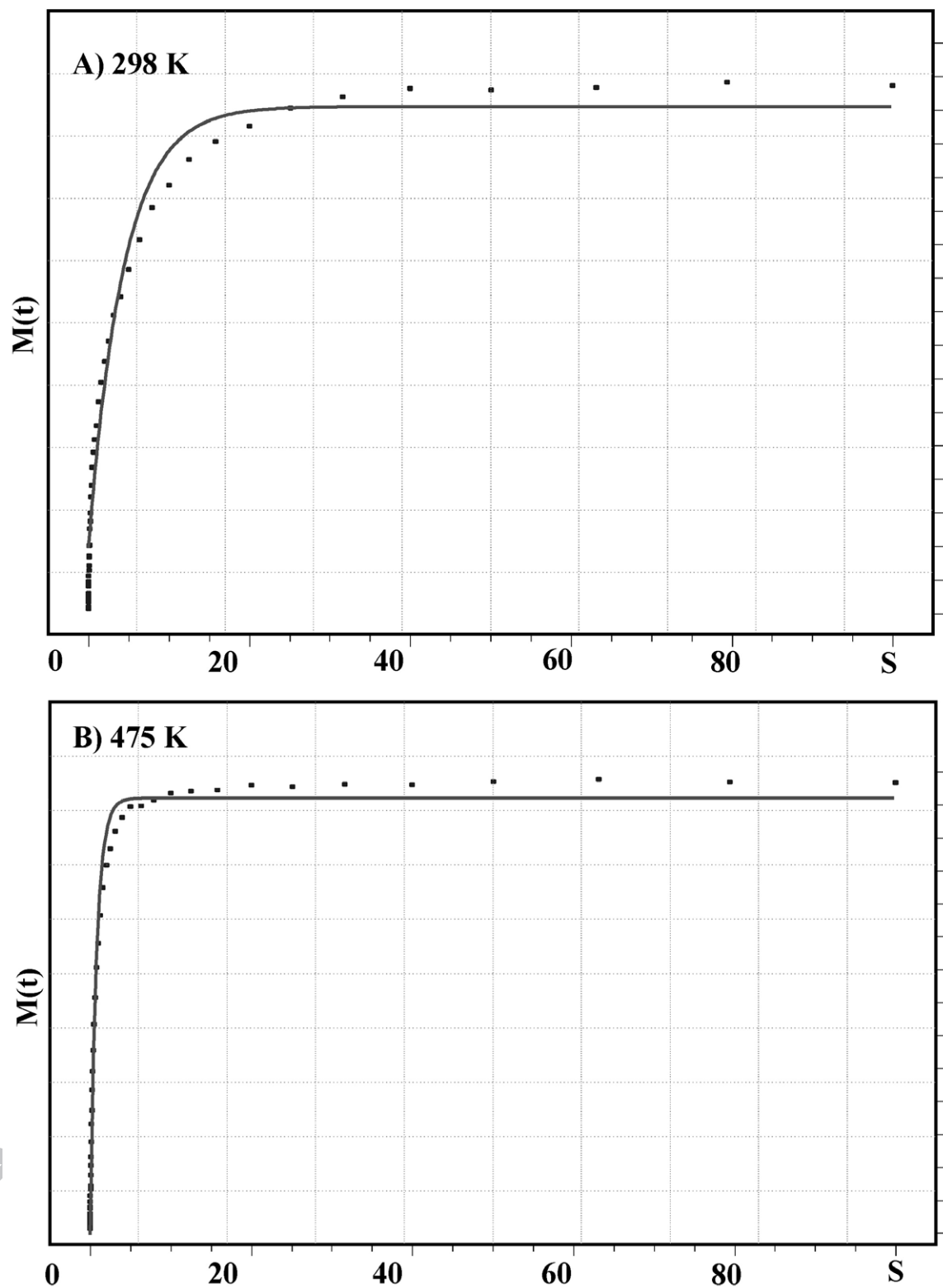
Figure 5: ^1\text{H} saturation-recovery data for the ^{15}\text{N} -enriched IRMOF-3 at 298 K (A) and at 475 K (B) plotted in arbitrary units. The smooth line in each is a fit to a single-exponential recovery.
