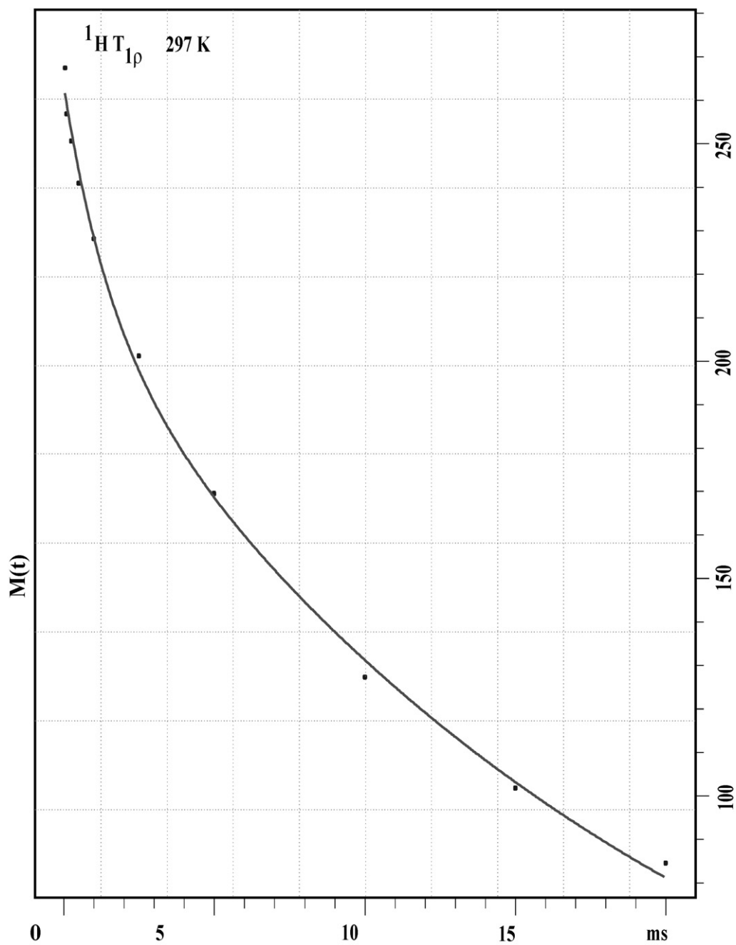
Figure 11: {}^1\text{H} spin-lattice relaxation data in the rotating frame ( T_{1\rho} ) for a sample of IRMOF-3 containing {}^{14}\text{N} at natural abundance plotted in arbitrary units. The temperature was 297 K.
