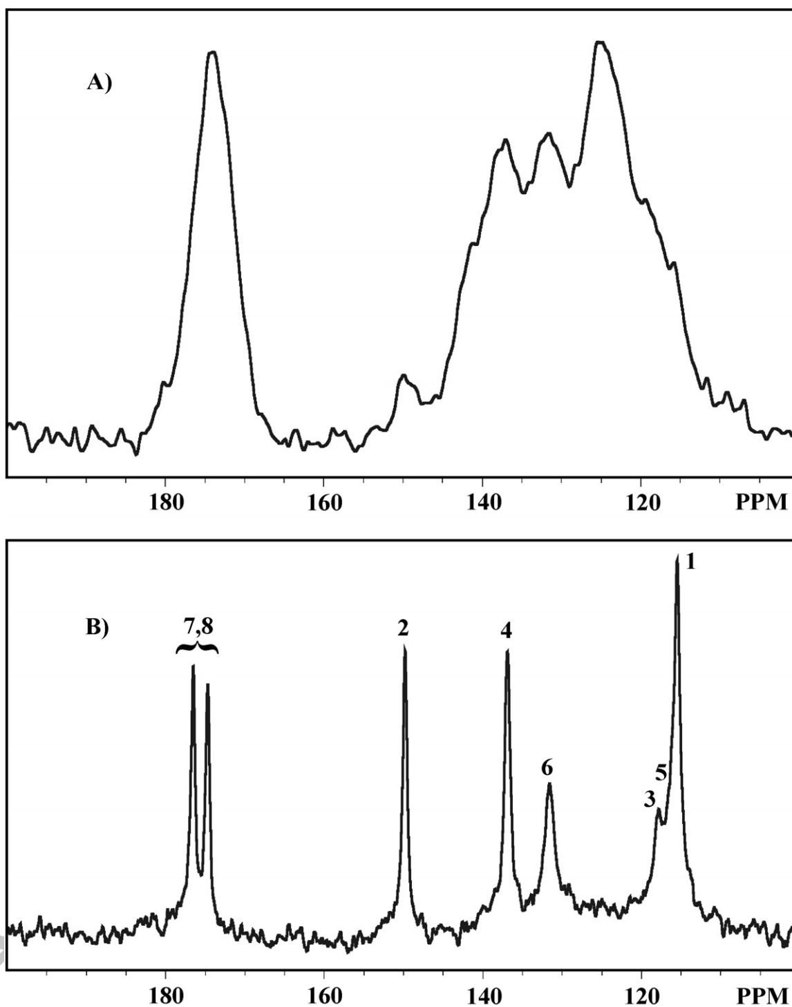
Figure 6: ^{13}\text{C} CP/MAS spectra of a sample of IRMOF-3 containing ^{14}\text{N} at the natural abundance (A) and of a sample highly enriched in ^{15}\text{N} (B). The ^{13}\text{C} spectral assignments given by the numerals in (B) refer to the scheme given in Figure 1(B).
