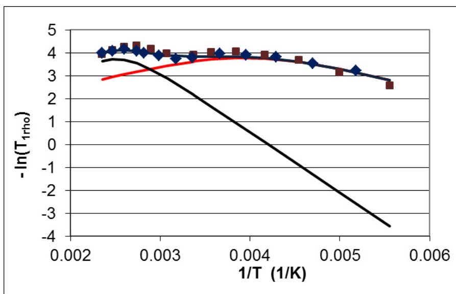
Figure 12: The negative of the logarithm of T_{1\rho} versus the inverse of the absolute temperature for IRMOF-3 containing ^{14}\text{N} at natural abundance. The experimental points are compared to a simulation, as described in the text ( \blacklozenge - enriched with ^{15}\text{N} ; \blacksquare - at natural abundance, 99.6% ^{14}\text{N} ). The lines show the predicted temperature dependence of the two contributions to the relaxation.
