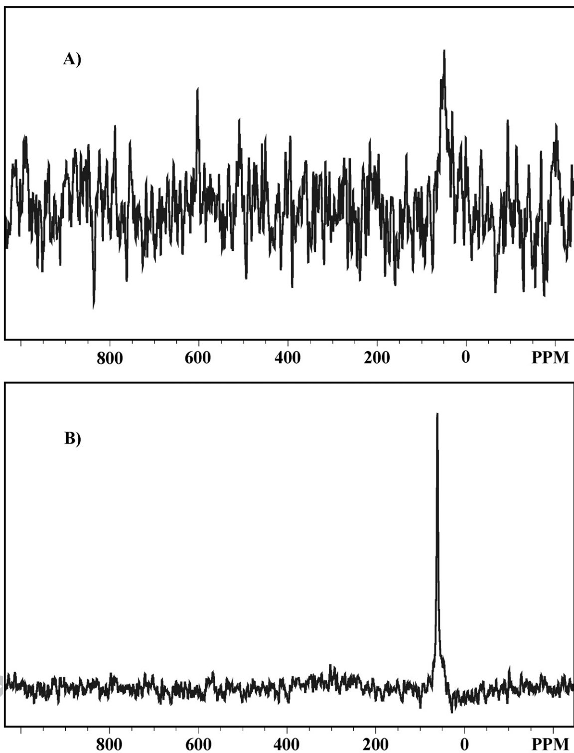
Figure 7: ^{15}\text{N} CP/MAS spectra of a sample of IRMOF-3 containing ^{14}\text{N} at natural abundance (A) and of a sample highly enriched in ^{15}\text{N} (B).
