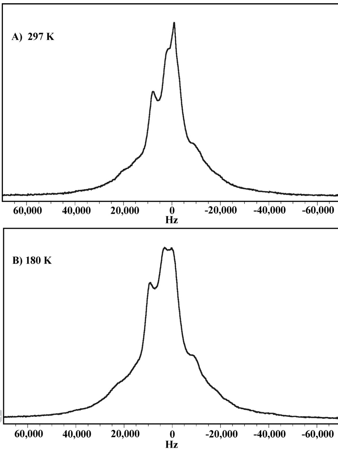
Figure 2: ^1\text{H} wide-line NMR spectra of IRMOF-3. The top spectrum (A) was acquired at 297 K, and the bottom (B) was acquired at 180 K.
