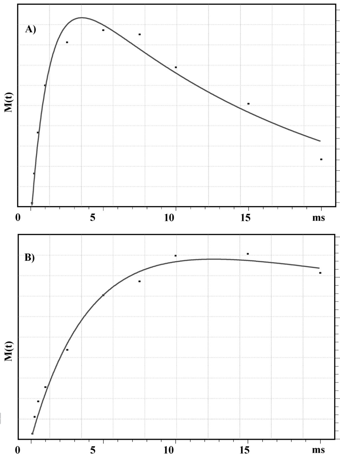
Figure 9: ^{13}\text{C} CP/MAS variable-contact data (magnetization plotted in arbitrary units) of the carboxyl resonance in a sample of IRMOF-3 containing ^{14}\text{N} at natural abundance (A) and of a sample highly enriched in ^{15}\text{N} (B). The smooth line in each is a fit of Mehring's variable-contact model. (See text.)
