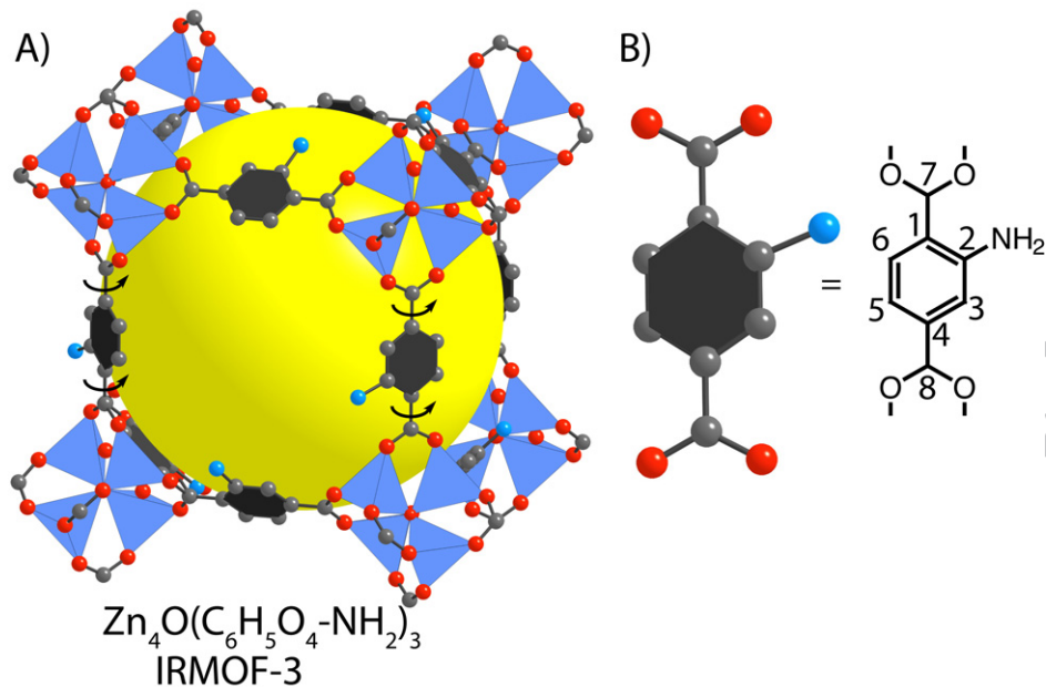
Figure 1: The structure of IRMOF-3 (A). The sphere represents the free volume within the framework. The numerical labeling in (B) is used to note ^{13}\text{C} spectral assignments.
