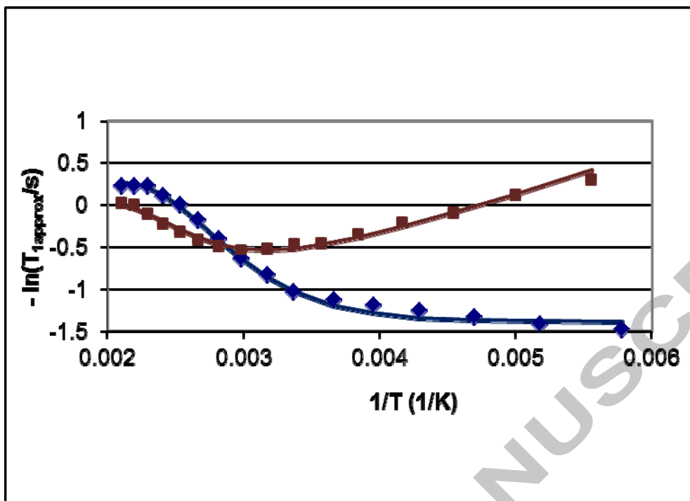
Figure 4: The negative of the logarithm of the ^1\text{H} spin-lattice relaxation time ( T_{1\text{approx}} ) as a function of the inverse temperature for IRMOF-3 ( \blacklozenge - enriched with ^{15}\text{N} ; \blacksquare - at natural abundance, 99.6% ^{14}\text{N} ). The solid lines are simulations, as described in the text.
