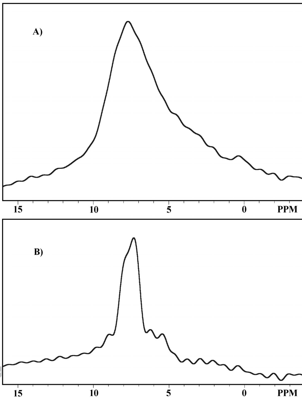
Figure 8: ^1\text{H} CRAMPS spectra of a sample of IRMOF-3 containing ^{14}\text{N} at natural abundance (A) and of a sample highly enriched in ^{15}\text{N} (B).
